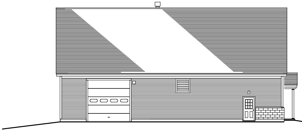
2 WEST ELEVATION
